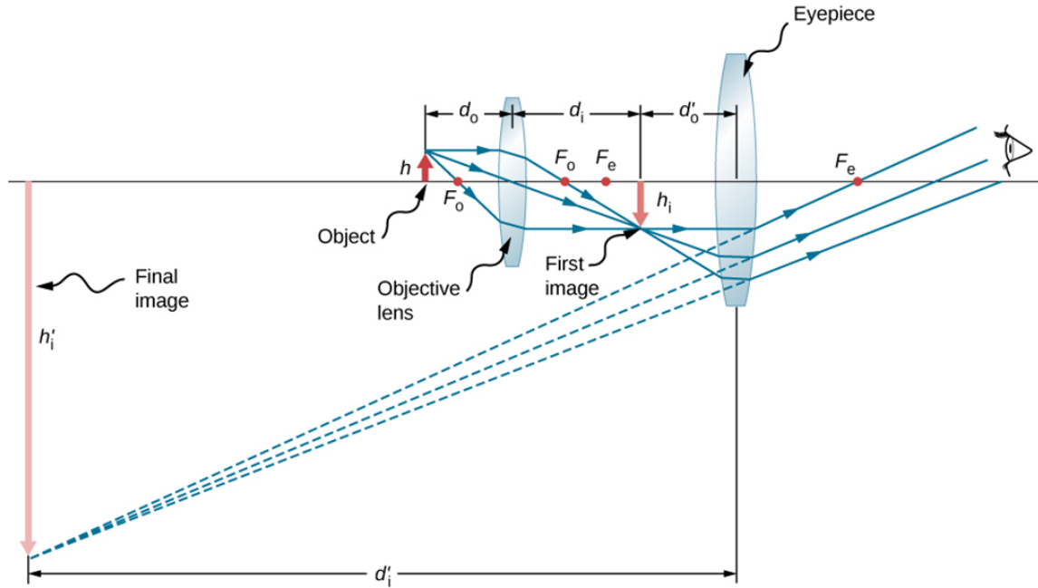
Figure 3.2.2.1 - Eyepiece Lens
