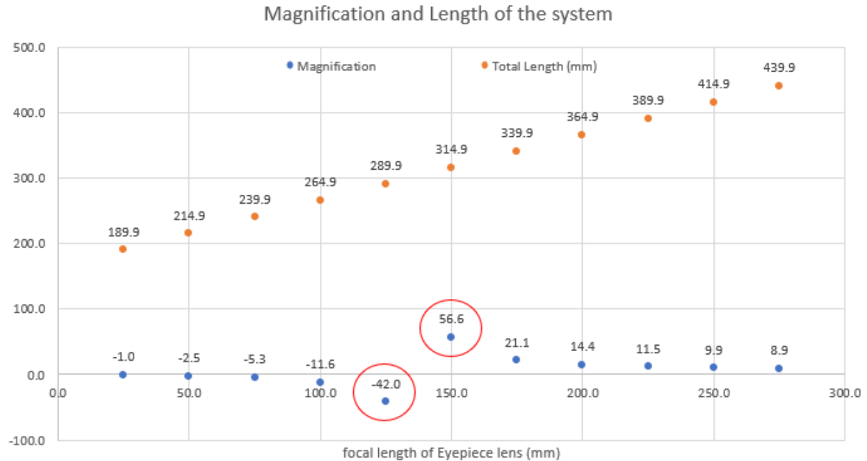
Figure 3.2.2.3 - Magnification and total setup length versus focal length of eyepiece lens
