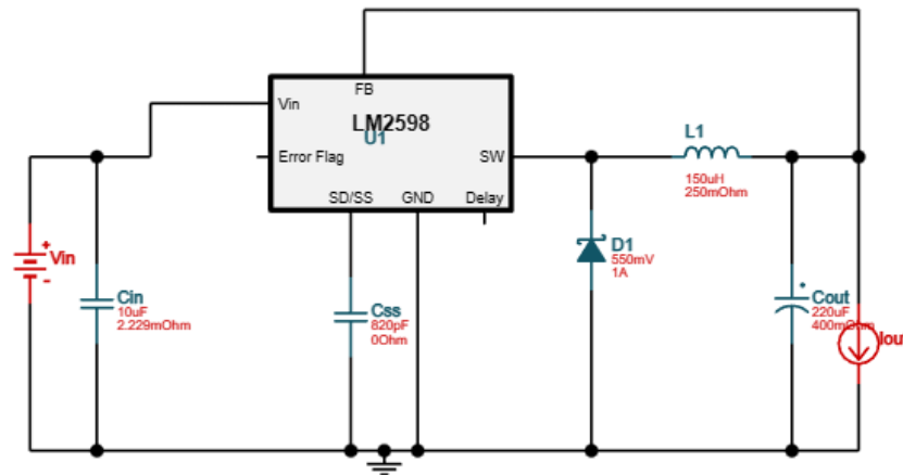
Figure 3.7.3 - LM2598 switching regulator design prototype
