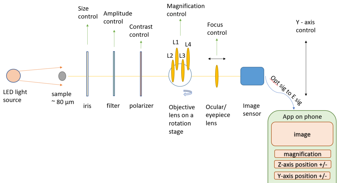
Figure 2.11.3 System design
