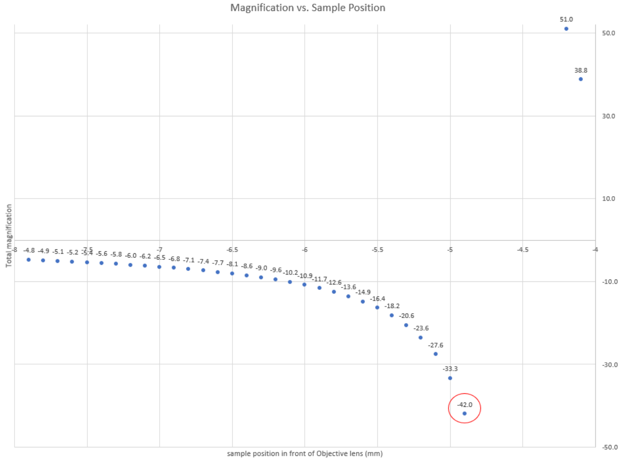
Figure 3.2.2.2 - Magnification versus sample position
