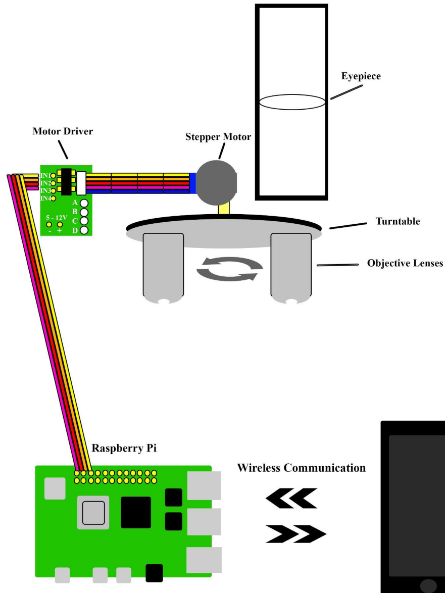
Figure 2.11.1 Turntable Design with Magnification level controlled with motors
