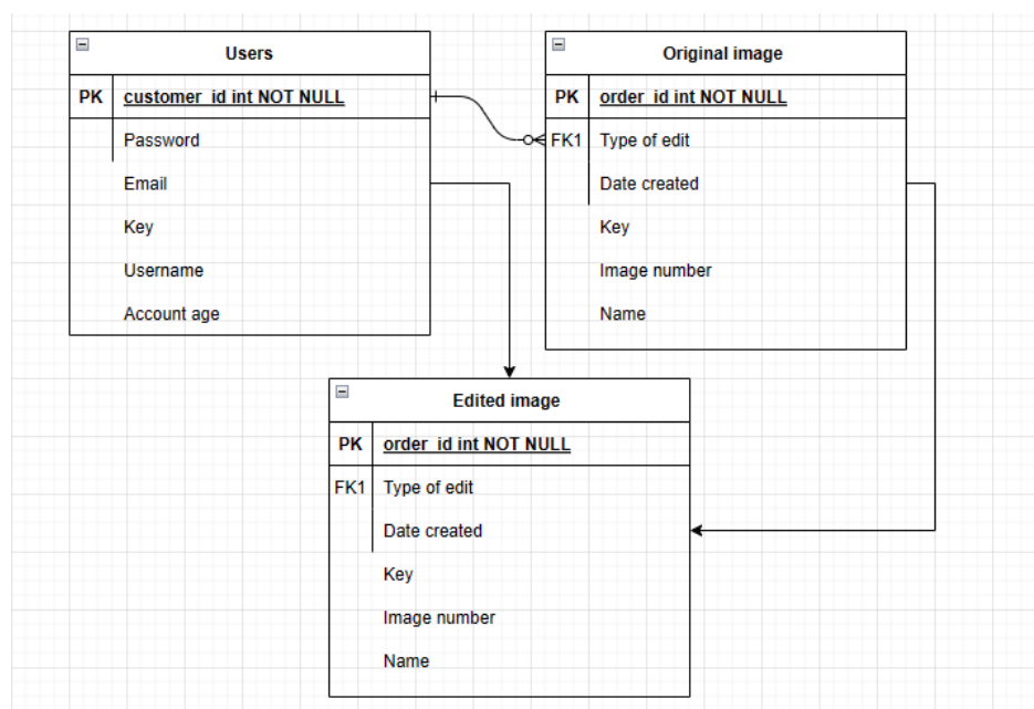
Figure 3.9.1.1 Sample ERD
